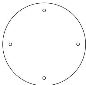
ø1100x10mm 1 x1PC
